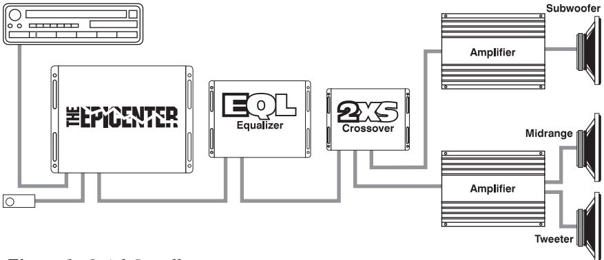
Figure 1: Quick Install
